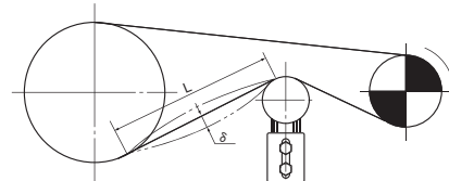
Fig. 7 Tensioner's anchored position
