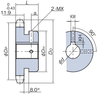
Hub with groove (10T – 11T)
