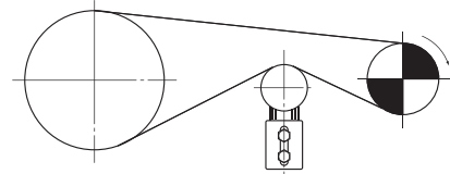
Fig. 5 Tensioner position (front)
