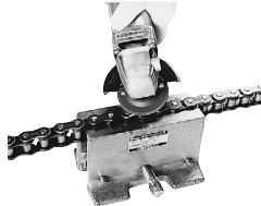
Fig. 2 Grinding the pin ends
