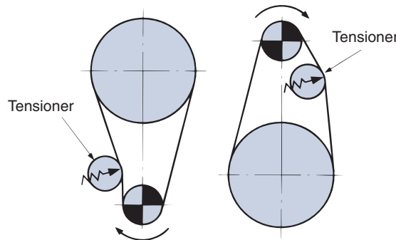
Fig. 22 Vertical transmission
