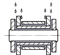
Fig. 10 Oiling locations
