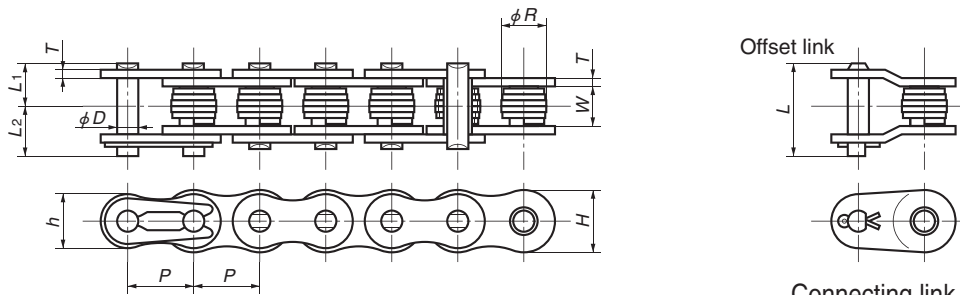
Connecting link RS80-SNS-1: Cotter pin-type
